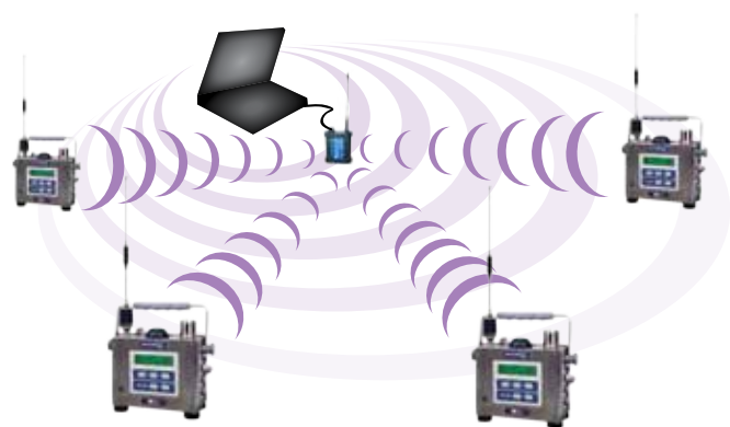
Wireless Area Monitoring Network with AreaRAE and RAELink2 Modem connected to a PC.
